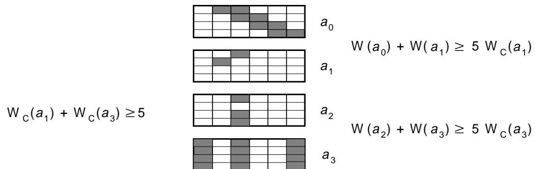
Figure 11: Illustration of Theorem 2.
