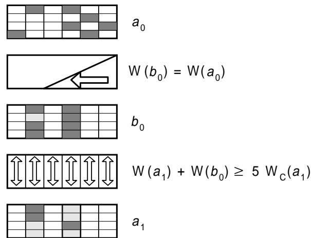
Figure 9: Illustration of Theorem 1 with Q = 2 .
